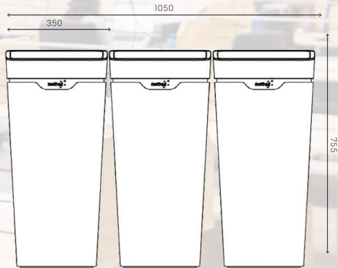
Measurements in mm Open height of closed lid bin - 1010mm
